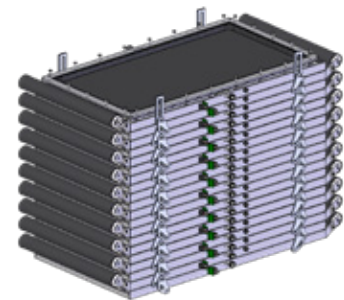
Roxia Plate Pack TP 32 16 2 45 C
